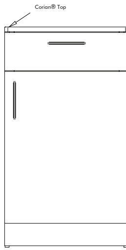
FRONT 1"=1"
