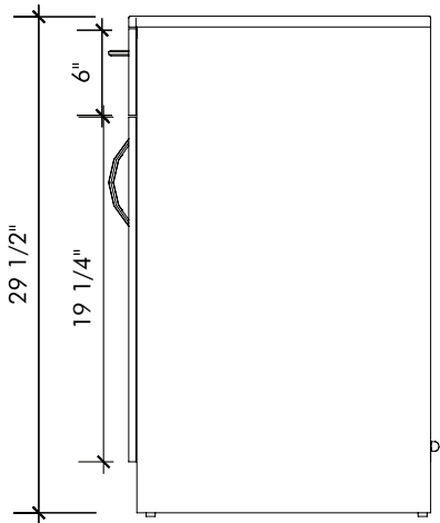
SECTION A 1"=1"
