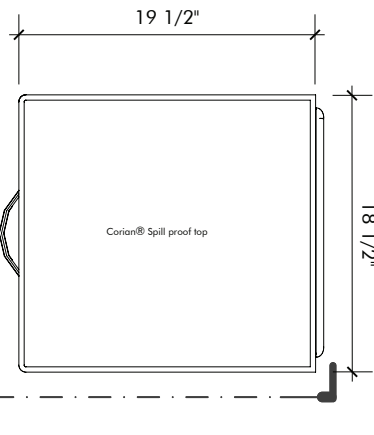
PLAN 1"=1"
