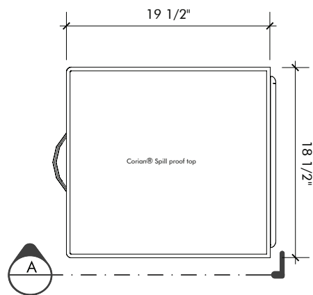
PLAN 1' = 1"
