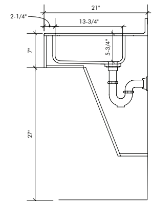
TYPICAL ADA LAYOUT TAMPER RESISTANT/FULLY ENCLOSED
