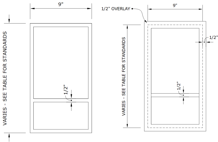
Front Elevation - Seamless
