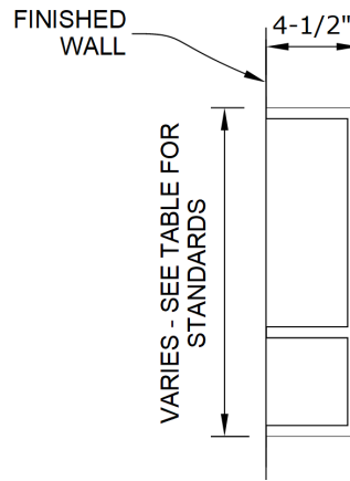
Side Section - Seamless
