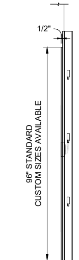
Side Elevation
