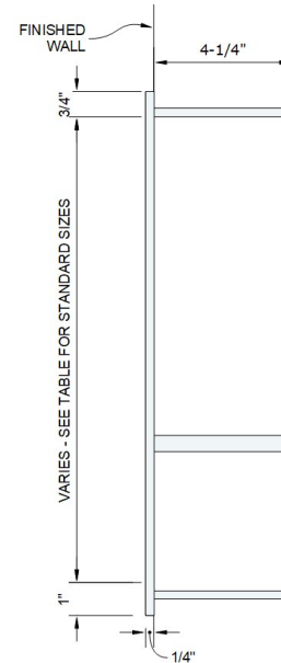
Side Section
