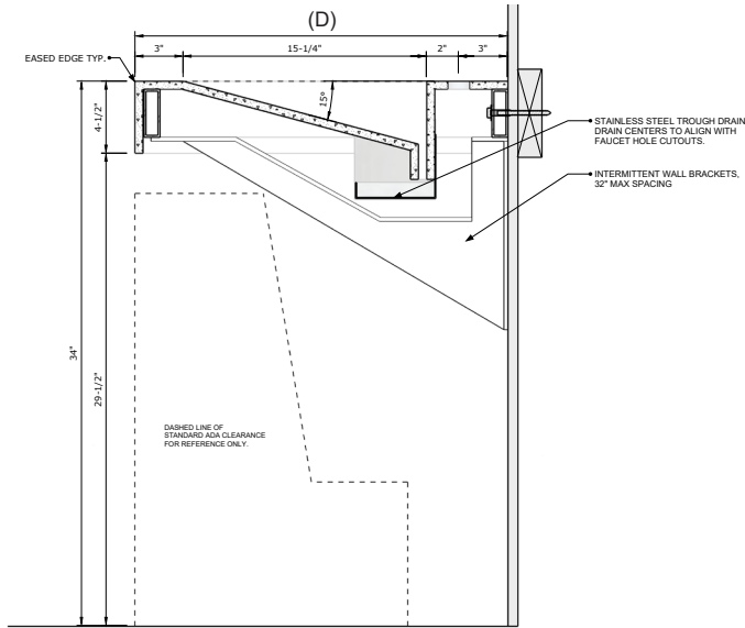
Side Cross Section
