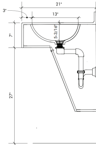
Tamper Resistant/ Fully Enclosed Section
