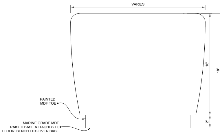
Section
