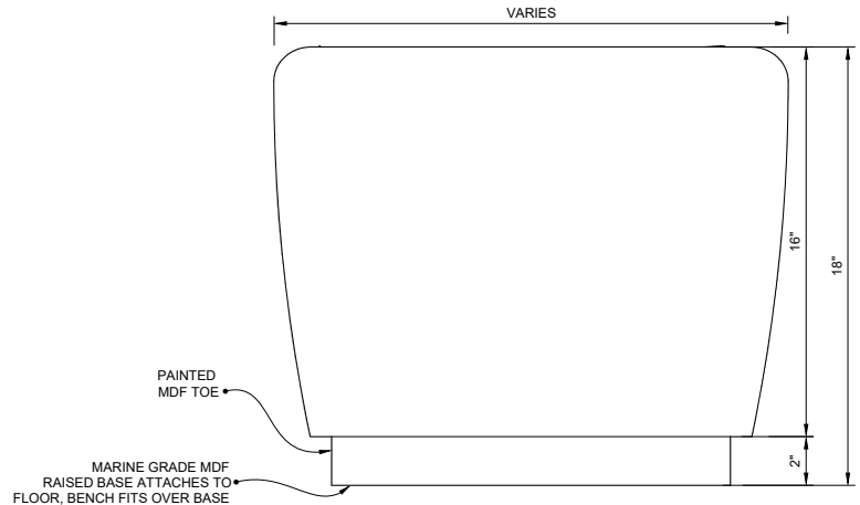
Section
