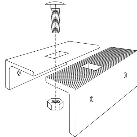
Attachment Detail
