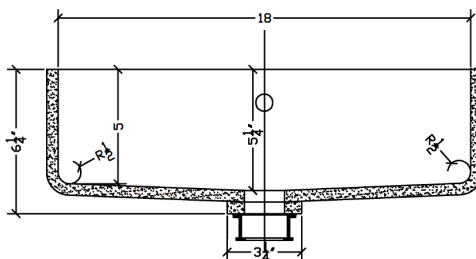
Front Cross Section
