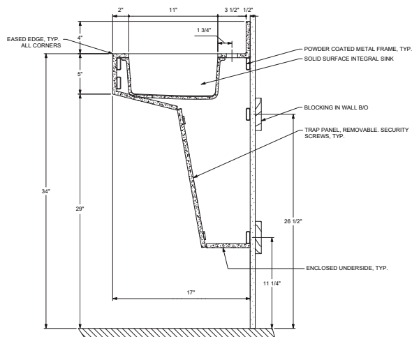
Side Cross Section
