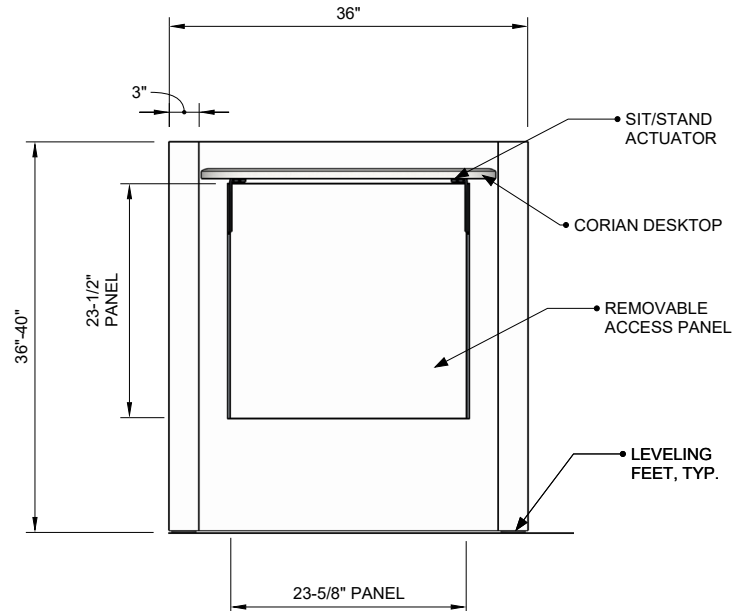
Elevation View
