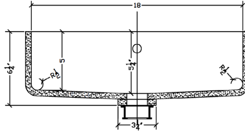
Front Cross Section
